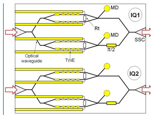
Figure 2: Schematic of the SSC-integrated and flip-chip ready twin-IQ MZ modulator PIC as basic active building block in the optical transmitter board. (TWE: Periodically capacity-loaded travelling wave electrode, SSC: spot size converter,
